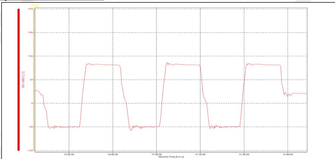
Figure 1. Testing record for Highly Accelerated Stress Screening
